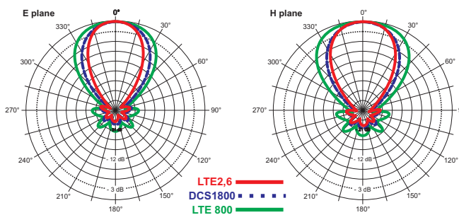
Radiation pattern of antenna: LAT - 56
